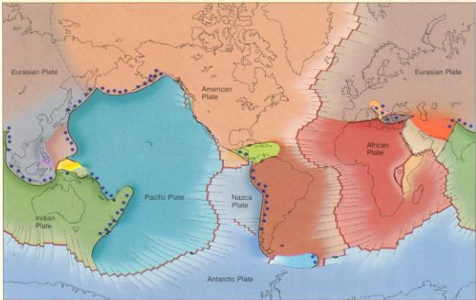
FIGURE 21.3 Seven major lithospheric plates.
